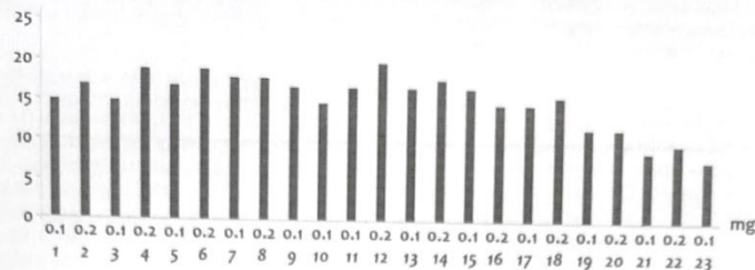
Fig. 2. Dependence of amplitude of muscle relaxation (mm) on the dose of control preparations and extracts of Cassia fistula L. (mg), namely, aqueous (abbreviation A in the legend), ethanol (EN) and ether (E) ones of various parts of the plant, namely, fruits (abbreviation F in the legend), leaves (L), shoots (S), bark (B): 1 – EL; 2 – EL; 3 – AL; 4 – ENL; 5 – ENL; 6 – EF; 7 – EF; 8 – ENF; 9 – ENF; 10 – AF; 11 – AF; 12 – ES; 13 – ES; 14 – ENS; 15 – ENS; 16 – AS; 17 – AS; 18 – EB; 19 – EB; 20 – AB; 21 – AB; 22 – ENB; 23 – ENB
